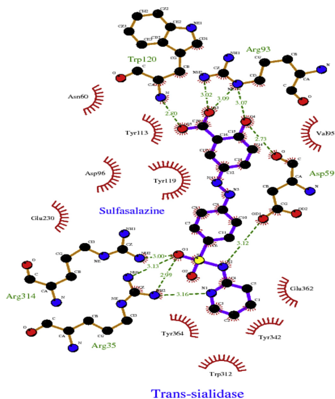
Fig. 5. Sulfasalazine docked on the trans -sialidase active site. Arcs with red lines represent amino acid hydrophobic contacts; green dashed lines represent hydrogen bonds. (For interpretation of the references to colour in this figure legend, the reader is referred to the web version of this article.)
