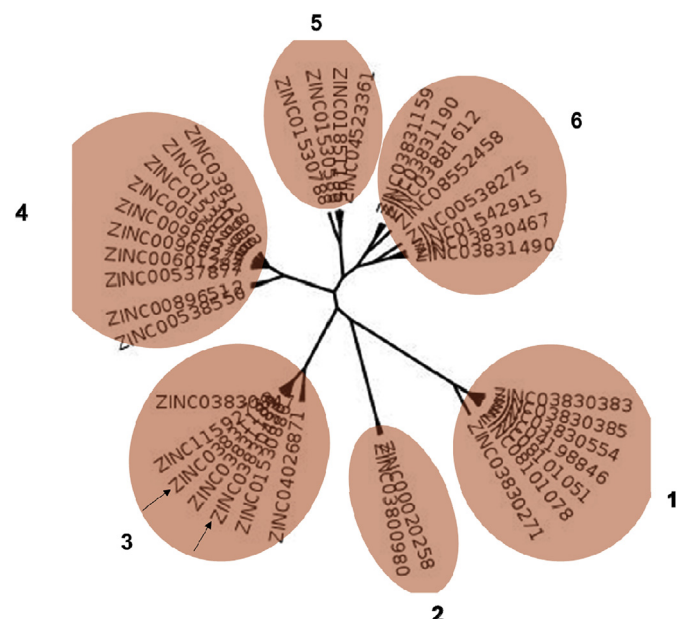
Fig. 2. Grouping patterns of the 38 top ranked FDA-drugs. The image was prepared using the Figtree software ( http://tree.bio.ed.ac.uk/software/figtree/ ).
