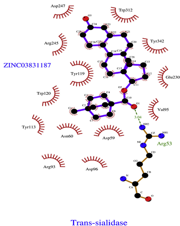
Fig. 1. The best ranked compound, ZINC0383118, docked on the Ts active site. Arcs with red lines represent amino acid hydrophobic contacts; green dashed lines represent hydrogen bonds. The 2D image was produced with LigPlot software [20]. (For interpretation of the references to colour in this figure legend, the reader is referred to the web version of this article.)
